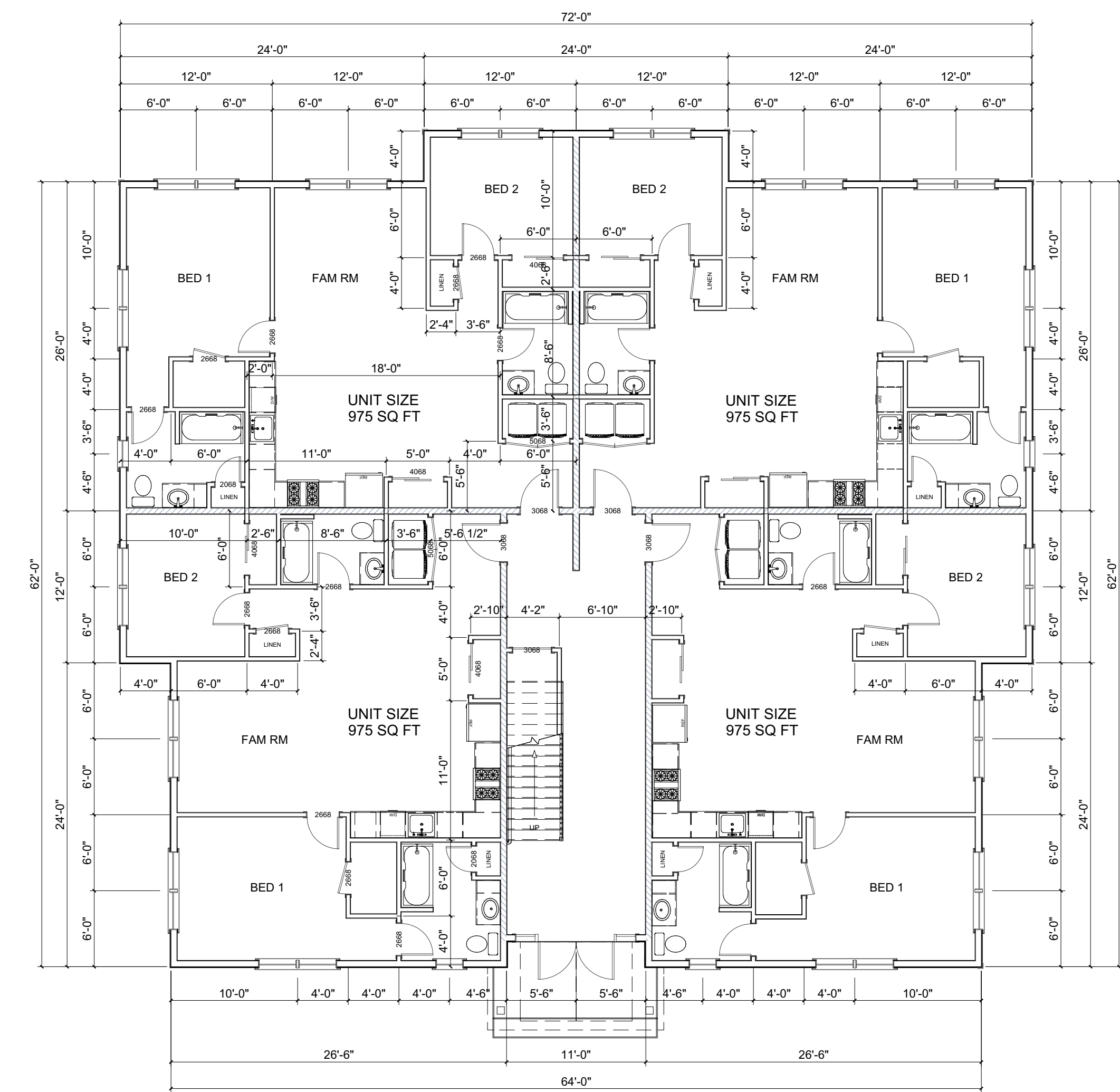
FLOOR PLAN
